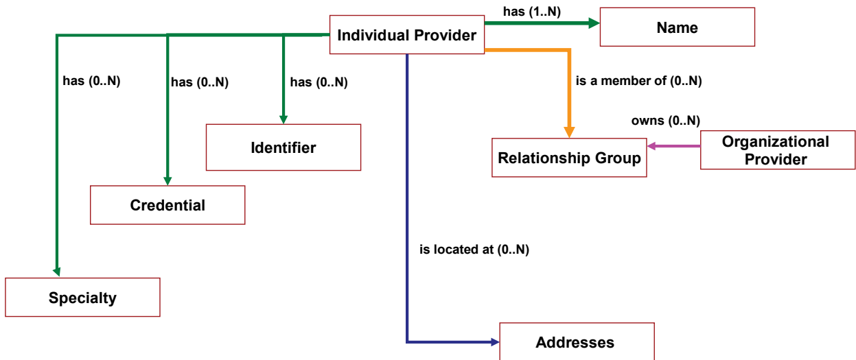
Figure 28.3.2.2-2: Individual Provider Entity and its Attributes
